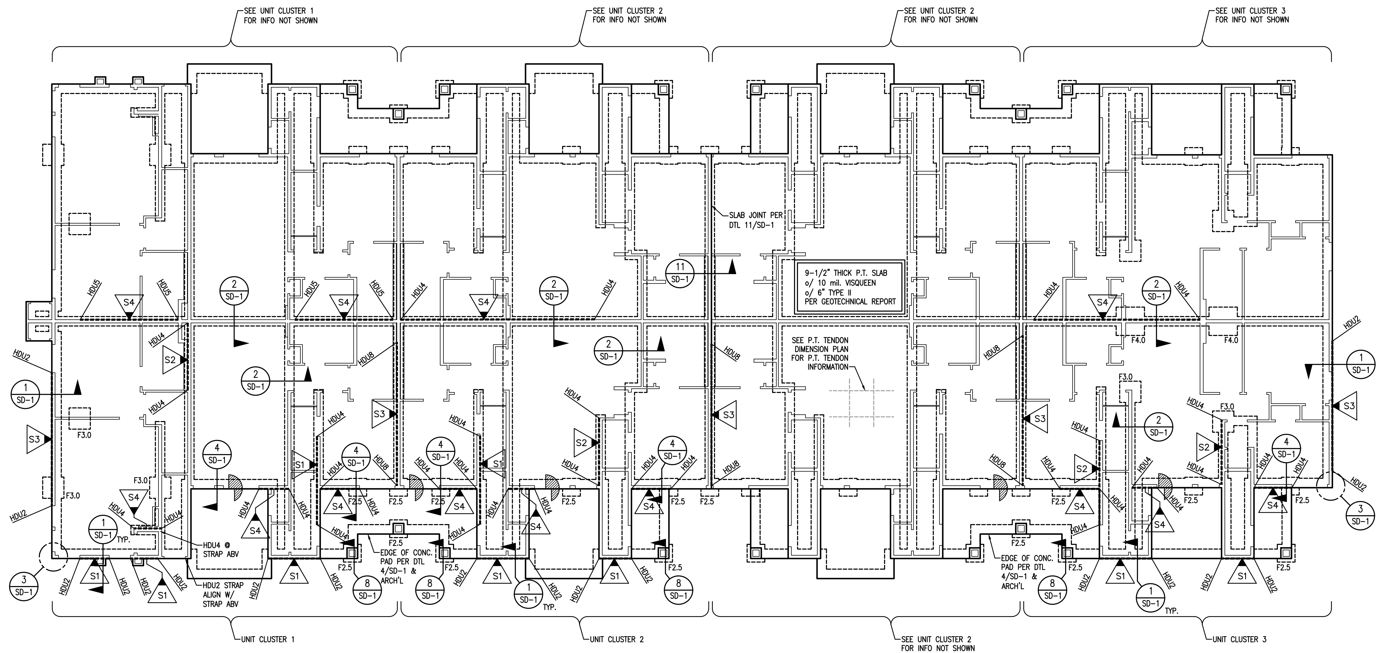
FOUNDATION PLAN BUILDING TYPE 1
