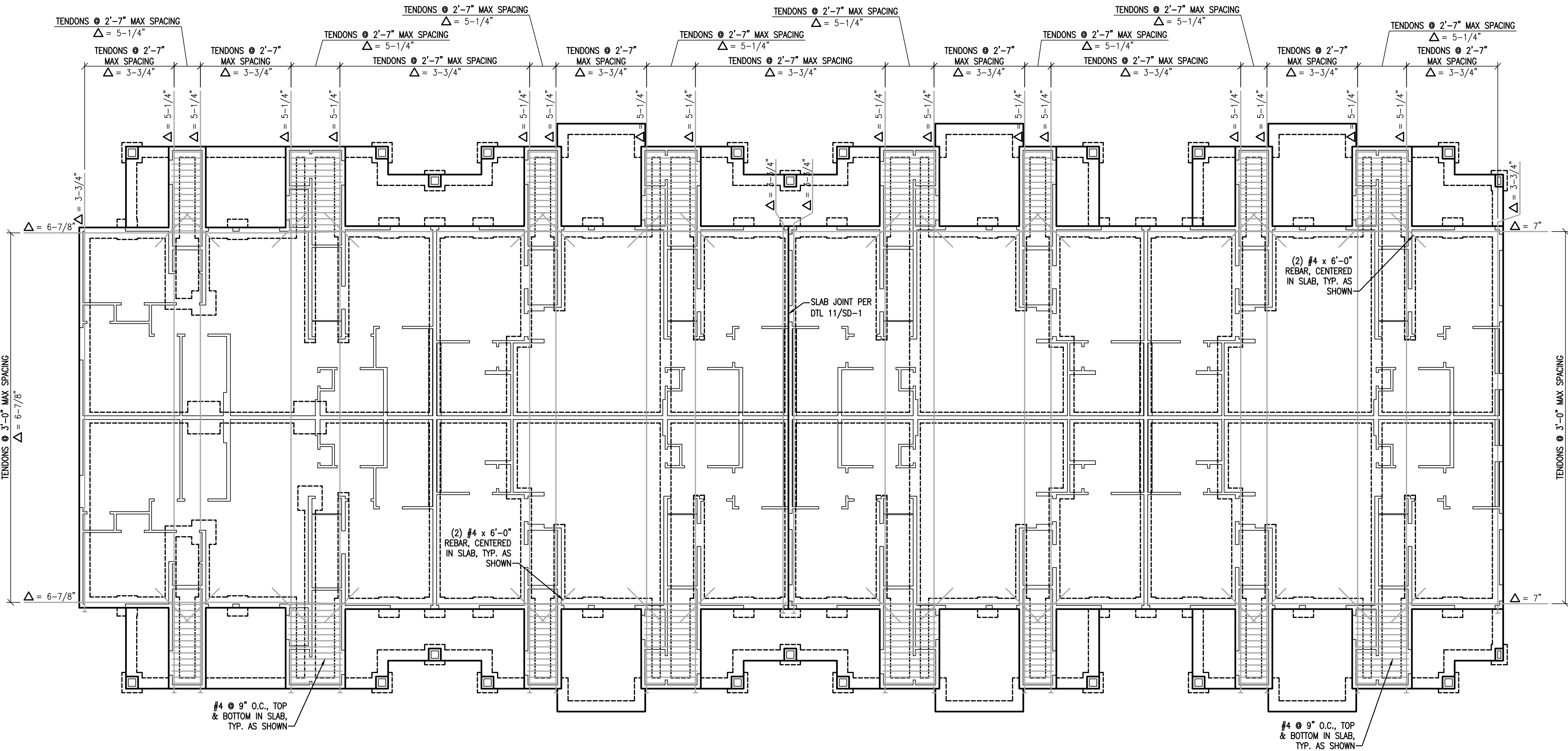
P.T. DIMENSION PLAN BUILDING TYPE 5
