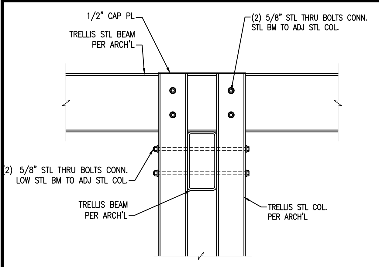
ELEVATION VIEW
