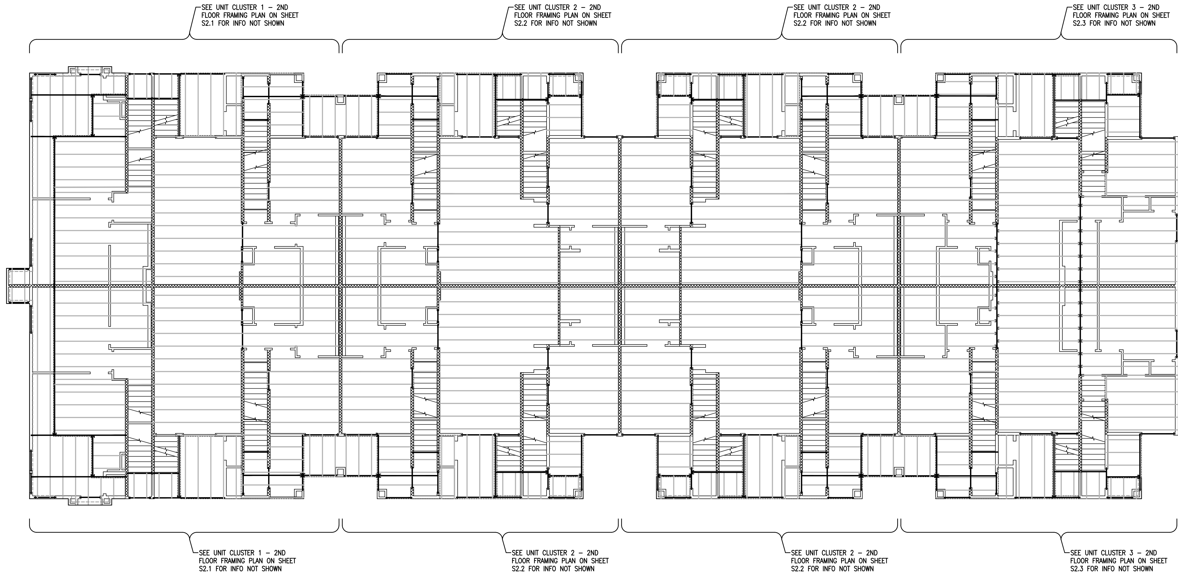
2ND FLOOR FRAMING PLAN BUILDING TYPE 1 1/8" = 1'-0"
