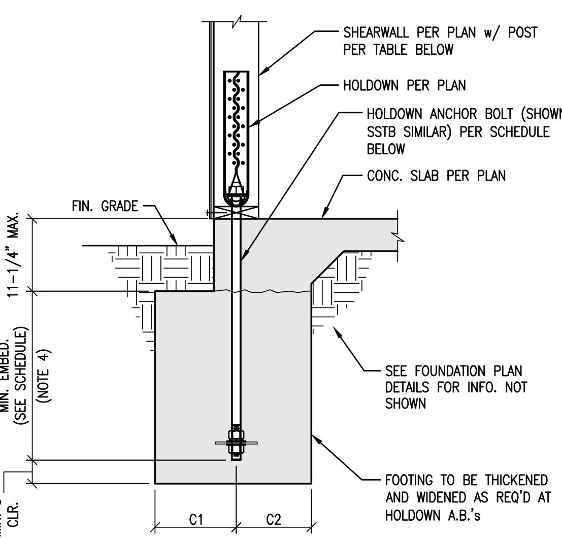
HDU HOLDOWN
