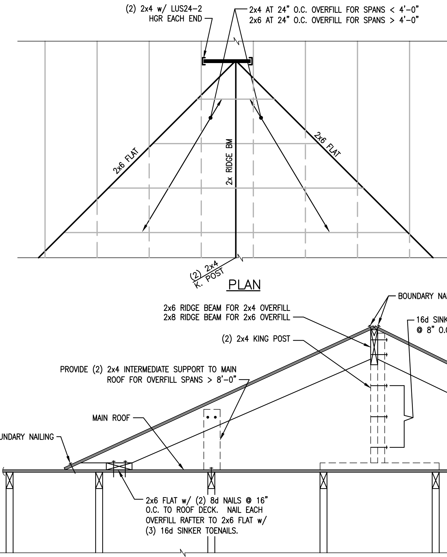
TYPICAL OVERBUILD
