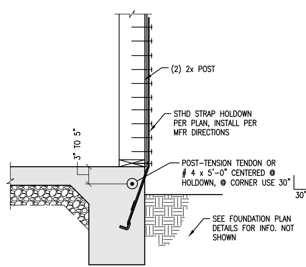
STRAP HOLDOWN
