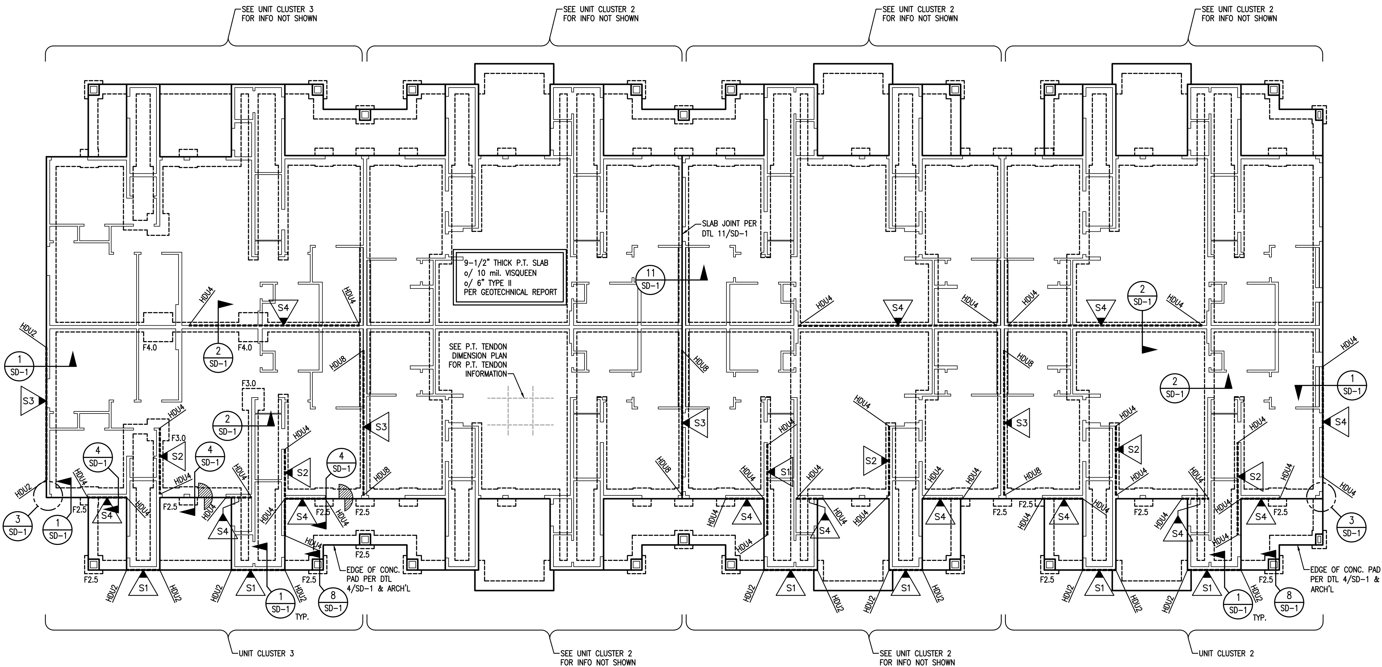
FOUNDATION PLAN BUILDING TYPE 5
