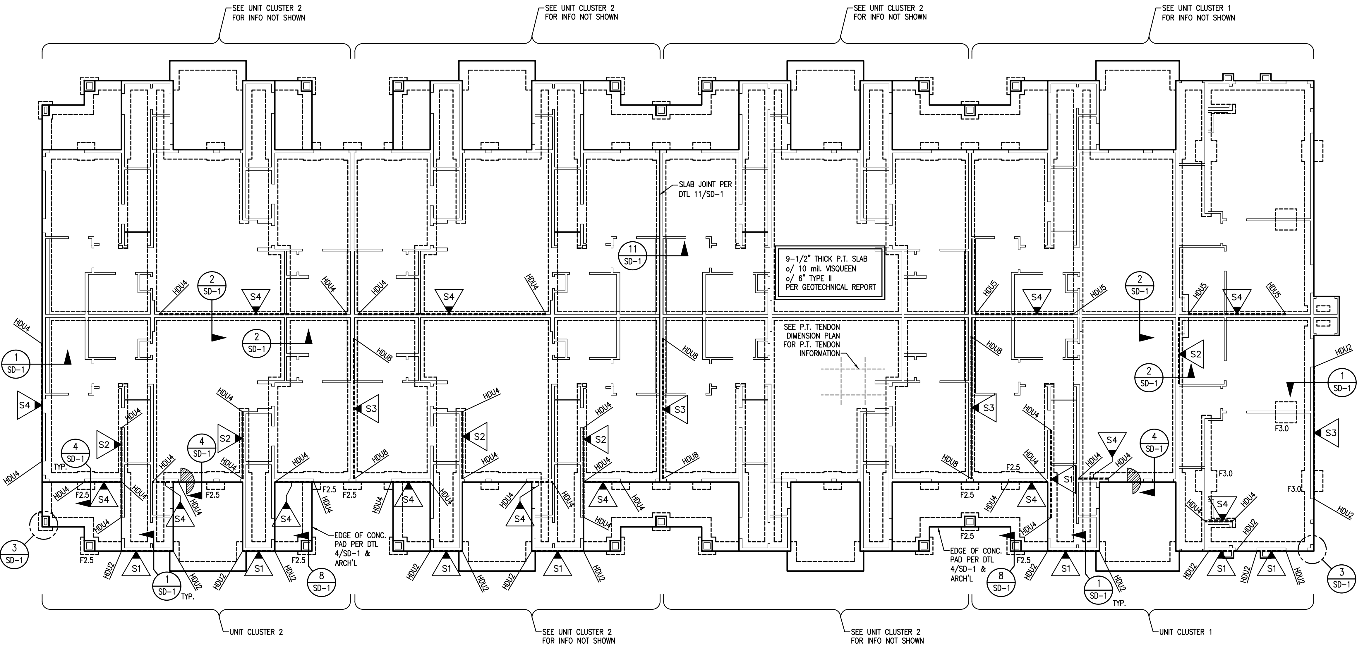
FOUNDATION PLAN BUILDING TYPE 3
