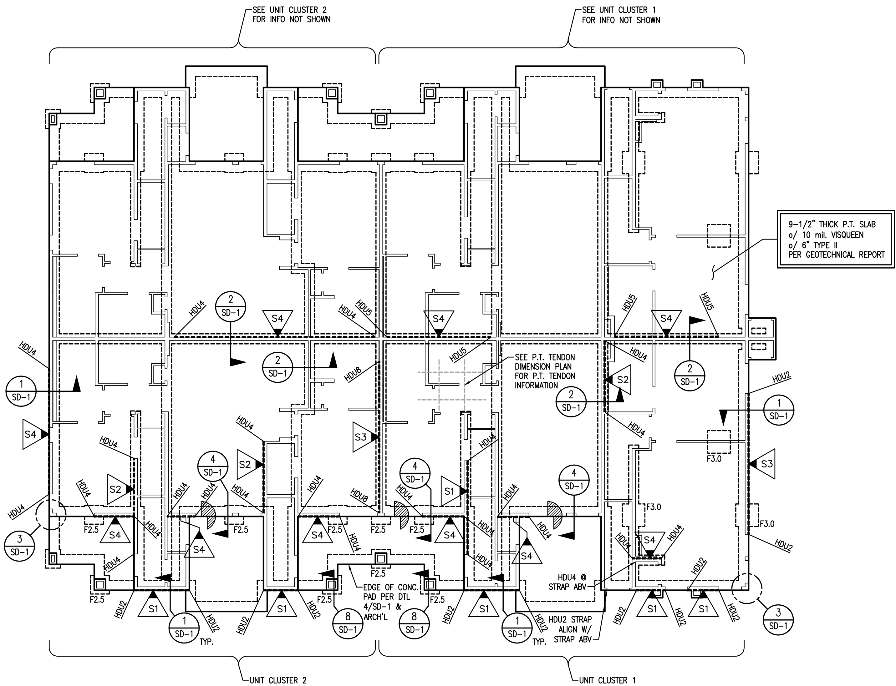
FOUNDATION PLAN BUILDING TYPE 4 1/8" = 1'-0"
