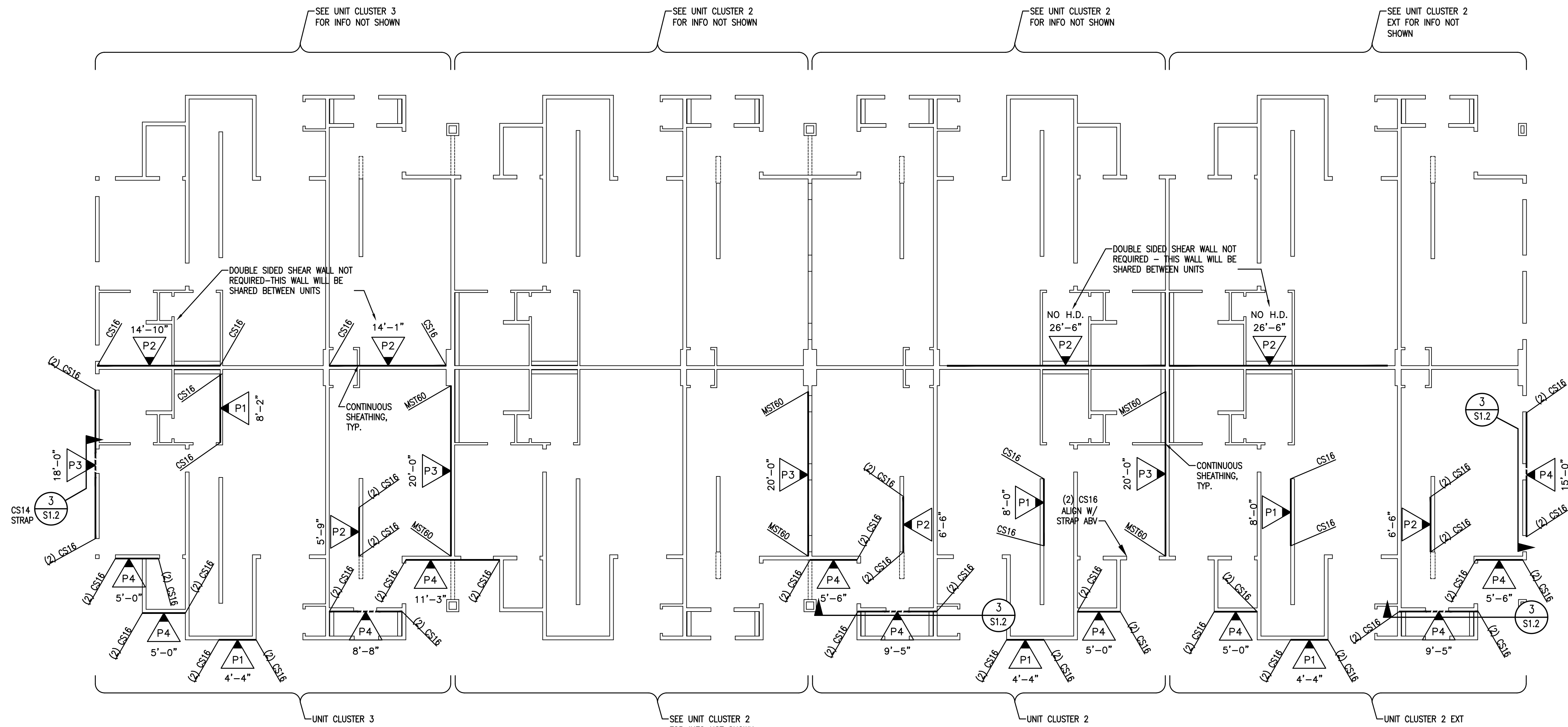
2ND LEVEL SHEAR WALL PLAN BUILDING TYPE 5 1/8" = 1'-0"
