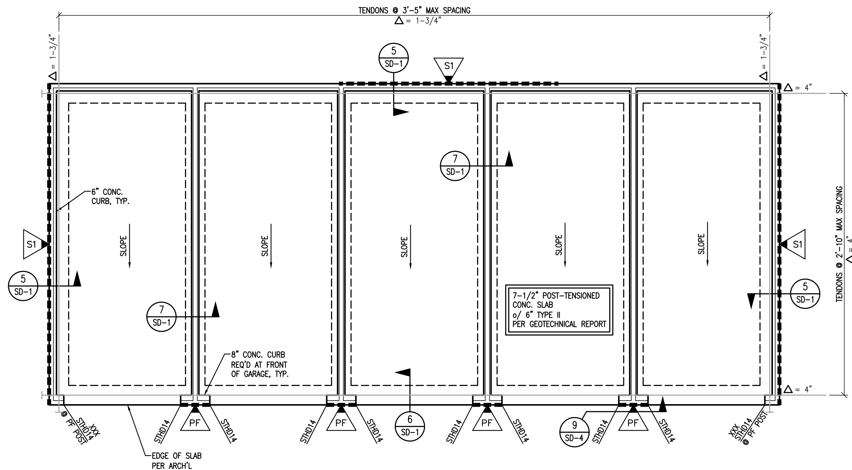
FOUNDATION PLAN GARAGE – ELEVATIONS A & B
