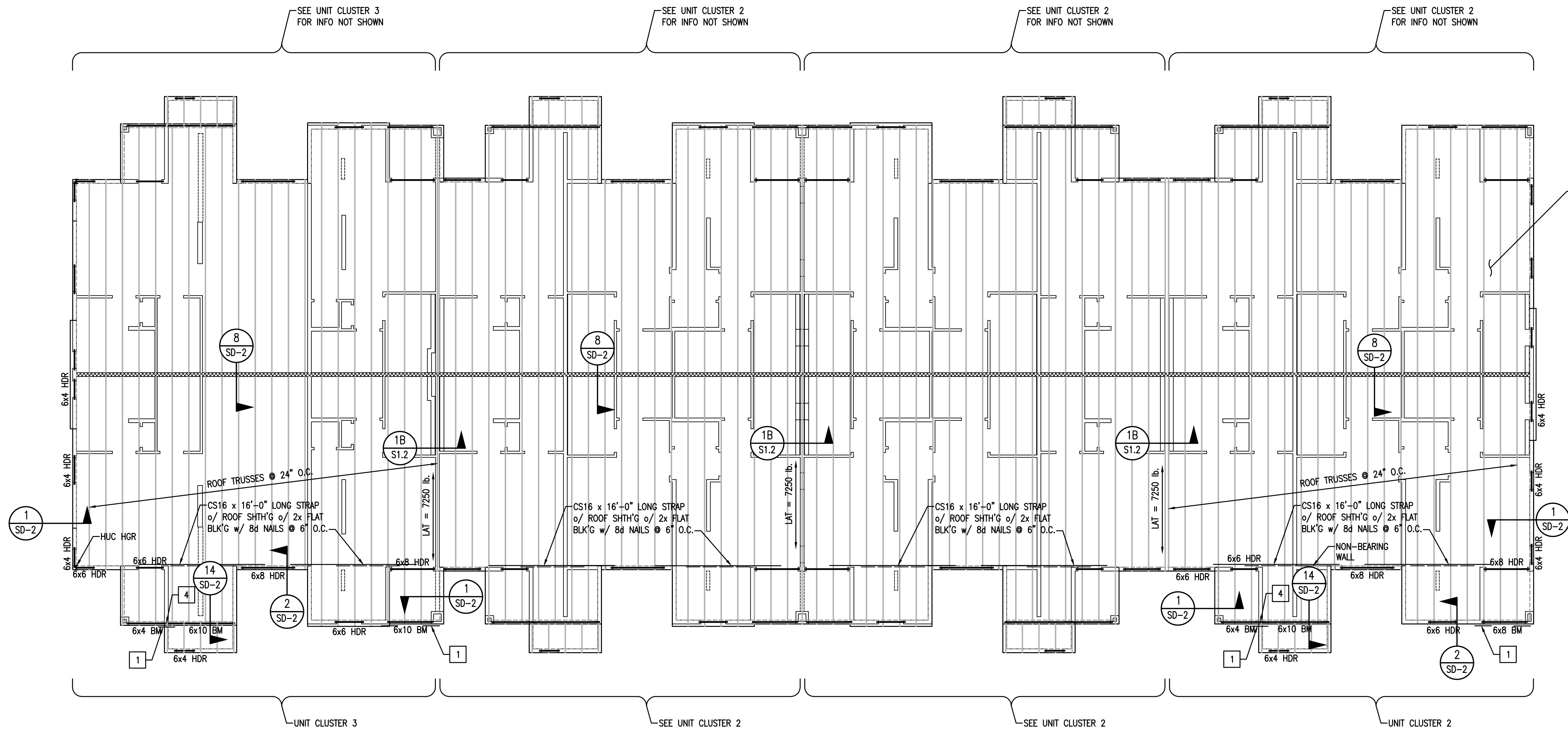
ROOF FRAMING PLAN BUILDING TYPE 5
