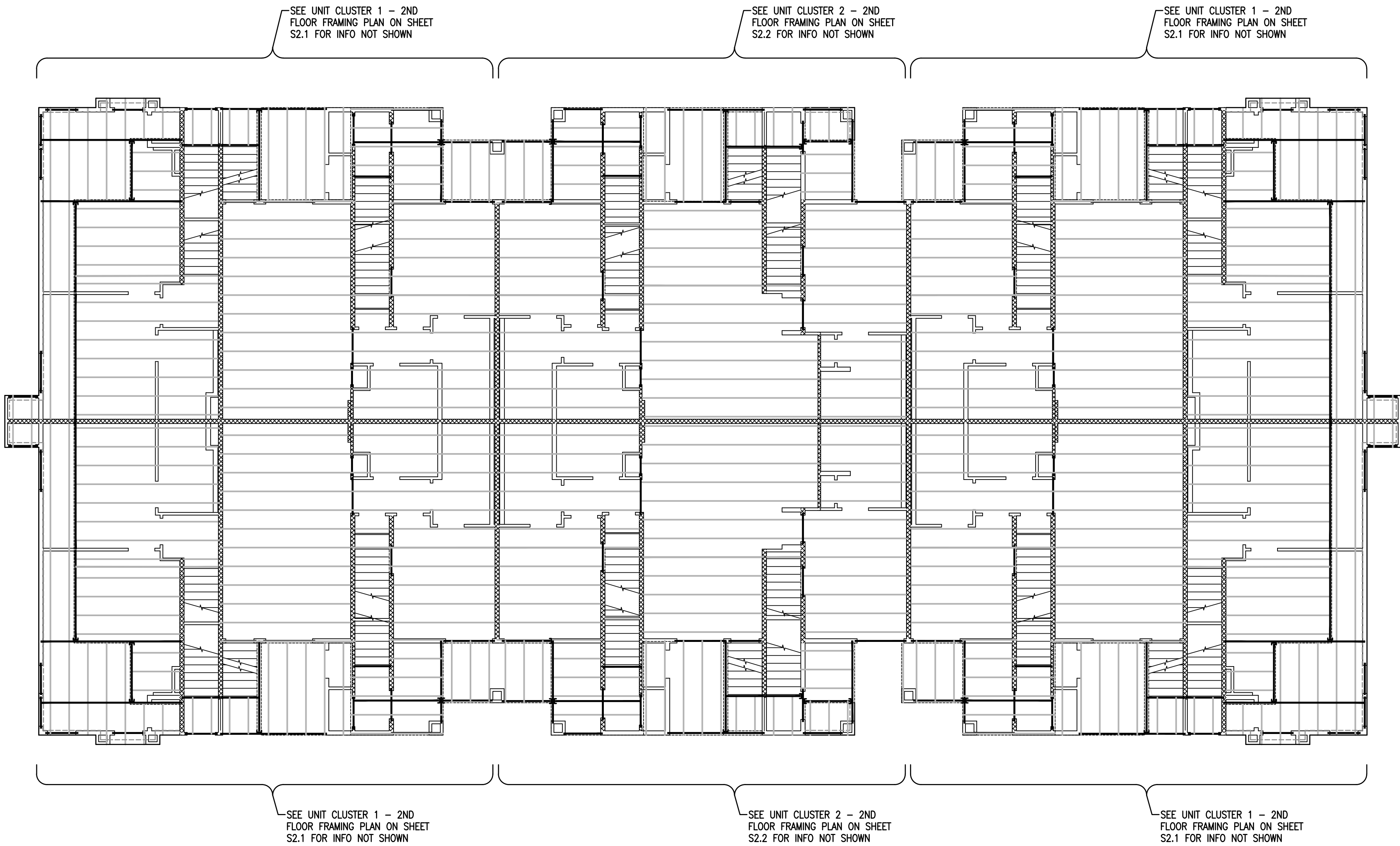
2ND FLOOR FRAMING PLAN BUILDING TYPE 2
