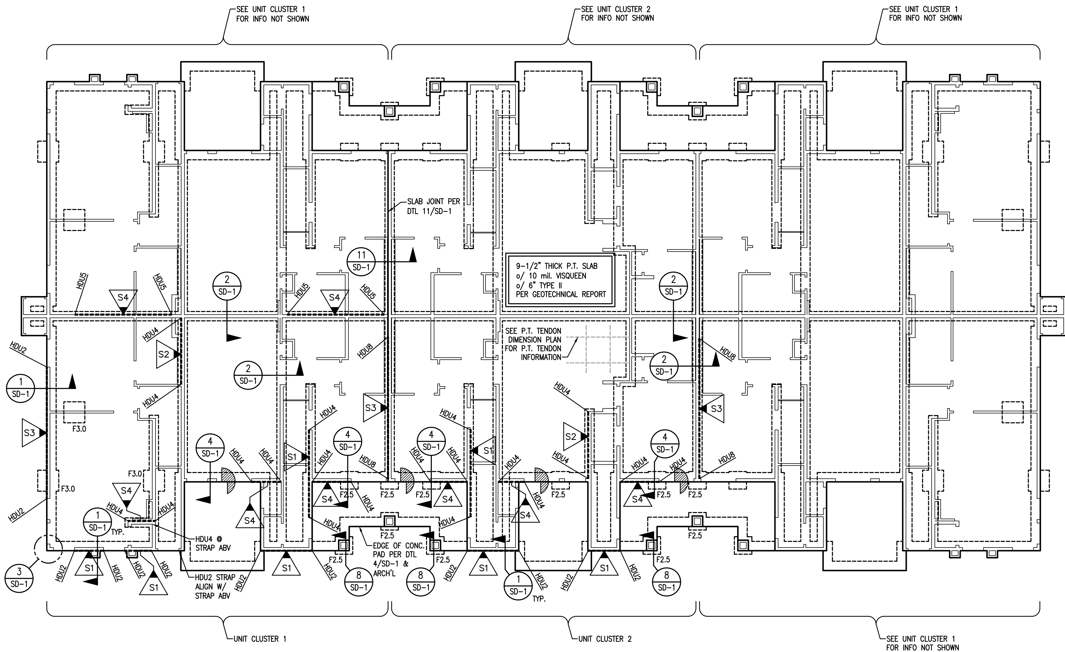
FOUNDATION PLAN BUILDING TYPE 2
